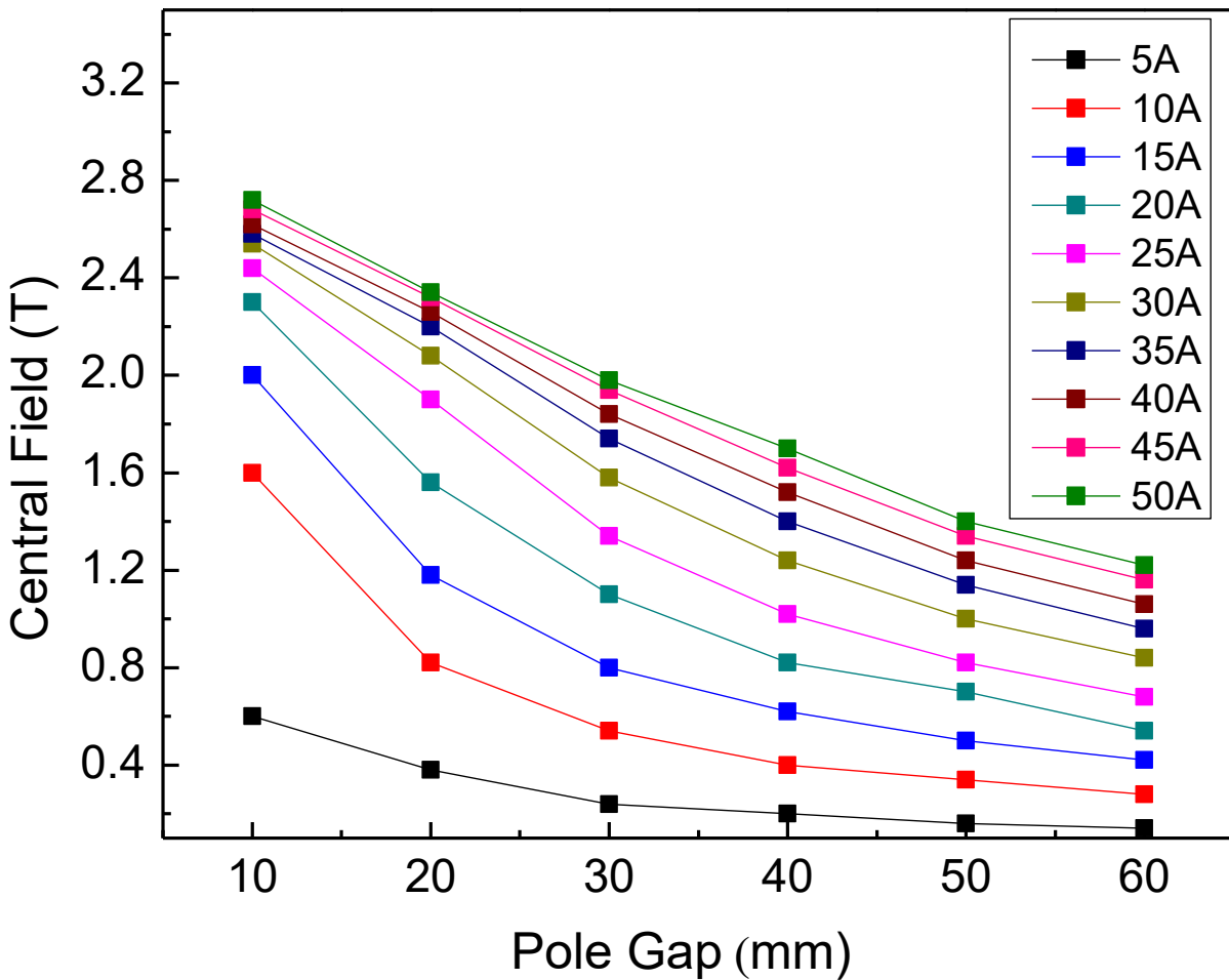
SB-175 Data for 60mm pole with Coils at Maximum Spacing
